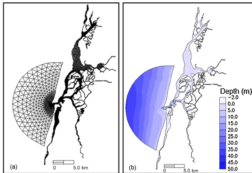
Fig. 4. Horizontal grid (a) and bathymetry (b) of the Ria de Aveiro.
