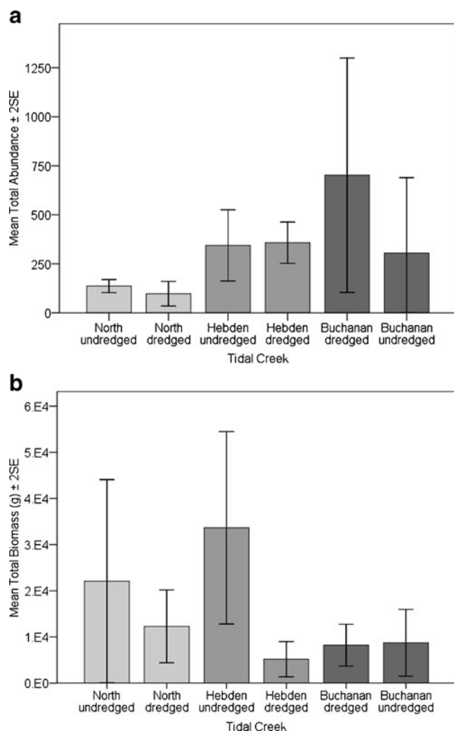
Fig. 3 Mean total a abundance and b biomass by tidal creek ( \pm 2SE, representing 95% confidence interval). No significant difference in abundance or biomass among creeks was observed in ANOVA analyses
